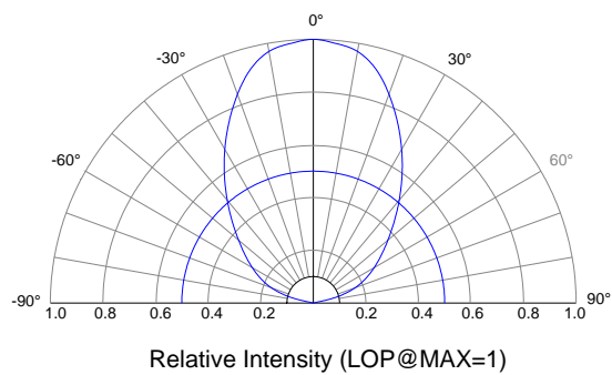
Beam Pattern
