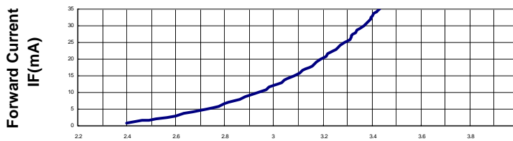
Forward Current vs Forward Voltage
