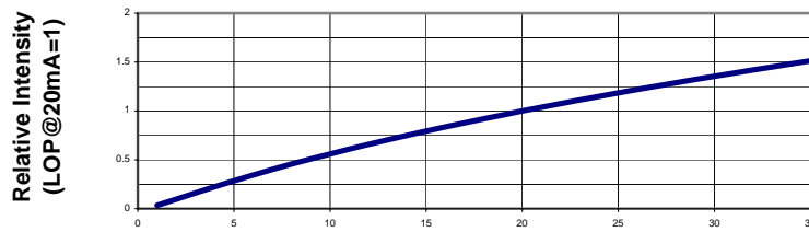
Relative Luminous Intensity vs Forward Current
