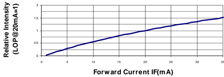
Relative Luminous Intensity vs Forward Current
