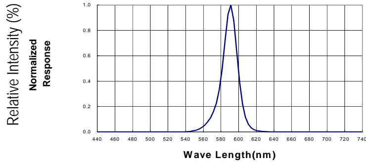
Relative Intensity vs. Wavelength Spectral Radiance (Peak @ 590nm)
