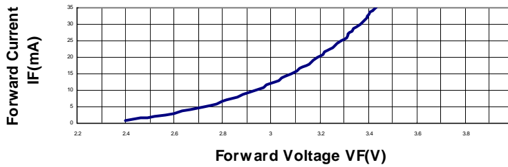
Forward Current vs Forward Voltage
