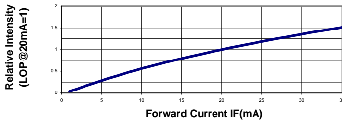
Relative Luminous Intensity vs Forward Current
